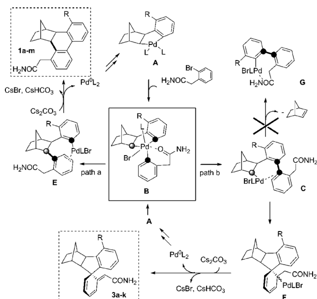
Scheme 3. Proposed mechanistic pathways.
